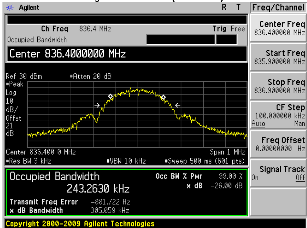
Figure Channel 189 (836.40MHz)
