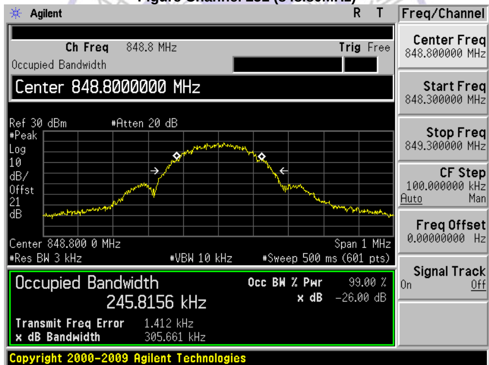
Figure Channel 251 (848.80MHz)
