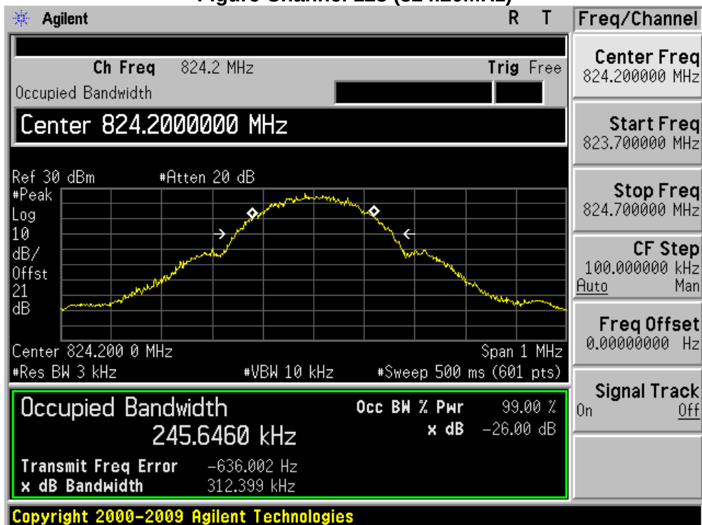
Figure Channel 128 (824.20MHz)
