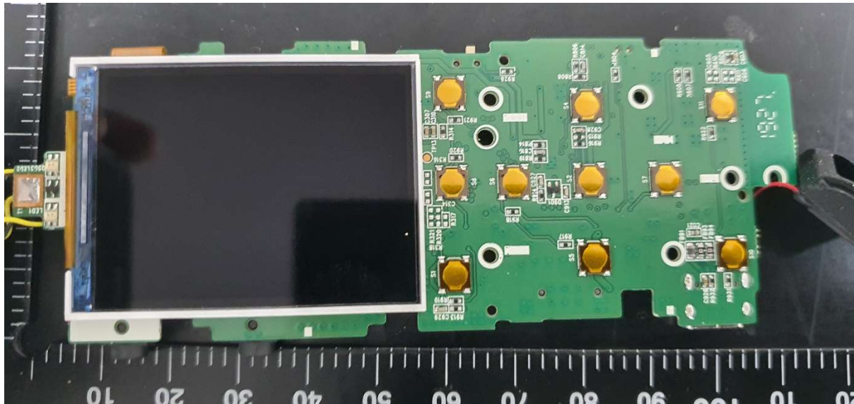
Main Board (rear)
