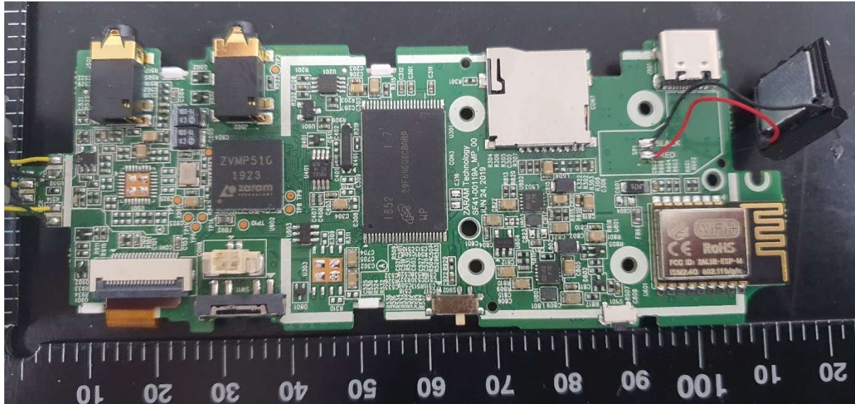
Main Board(Front)
