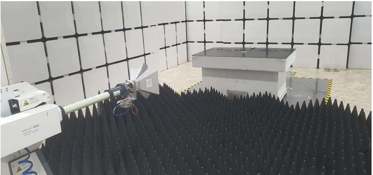
Test Setup
