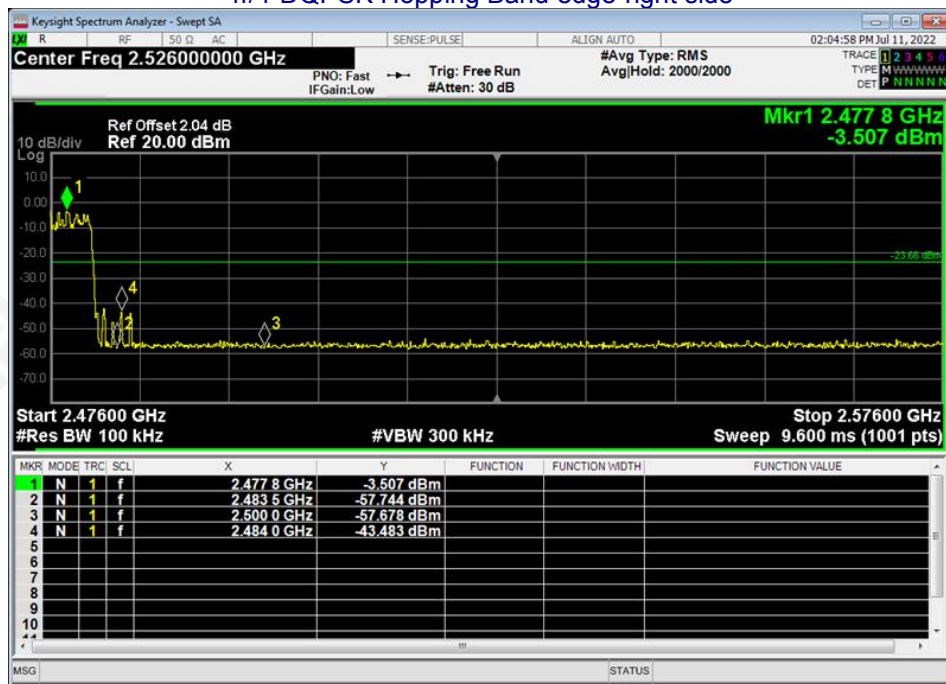
\pi/4 -DQPSK Hopping Band edge-right side
