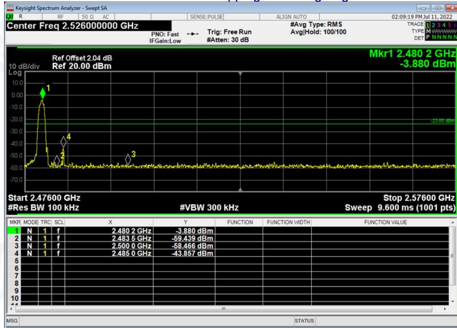
\pi/4 -DQPSK No-hopping Band edge-right side
