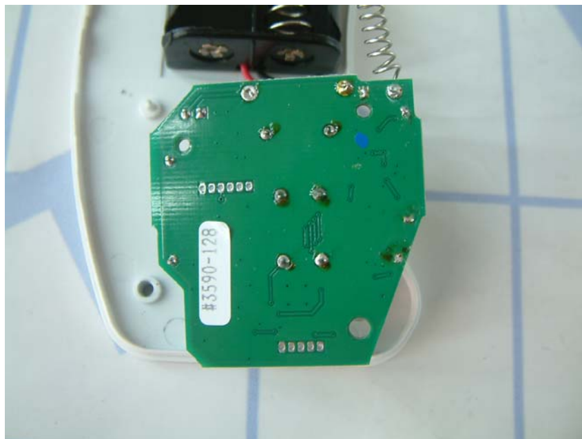
PCB view-2
