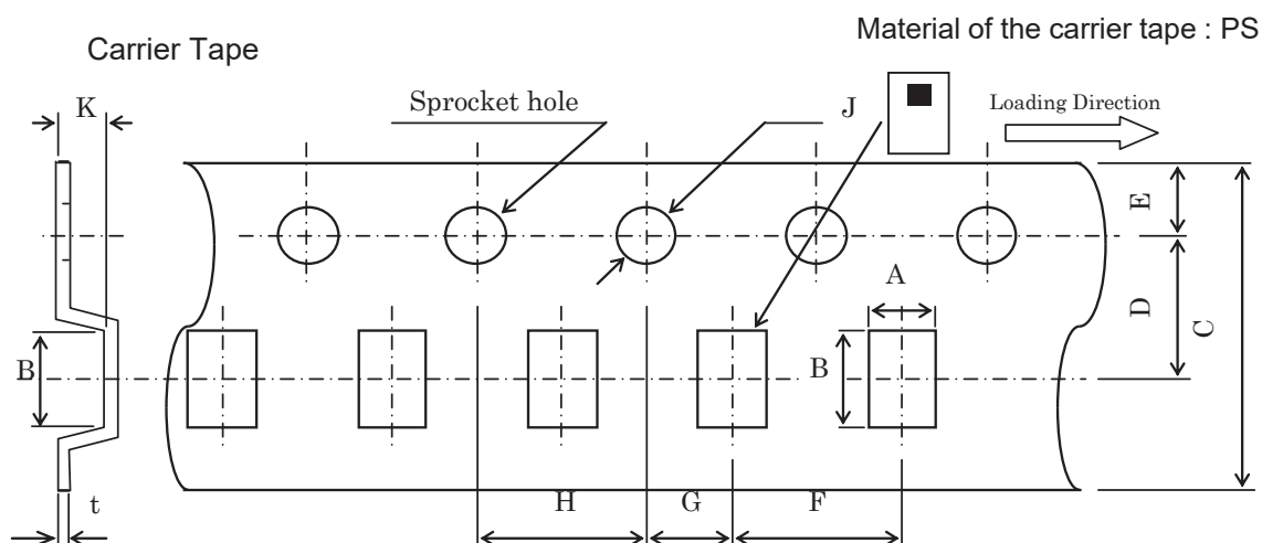
Dimensions (mm)
