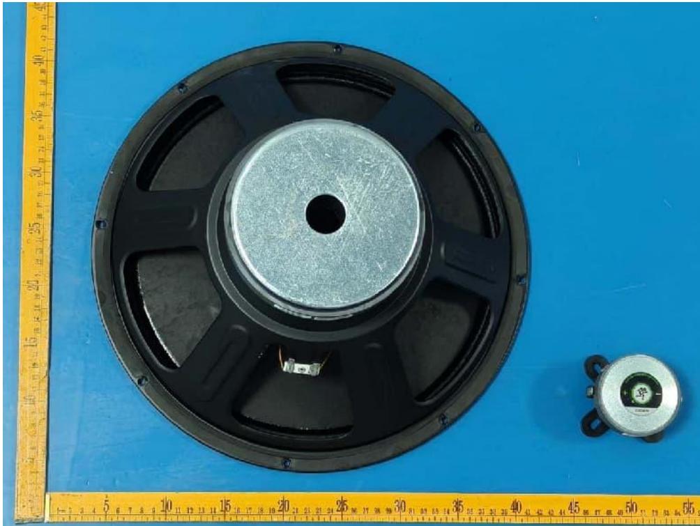
Horn view of unit (Model: THUMP15v4)
