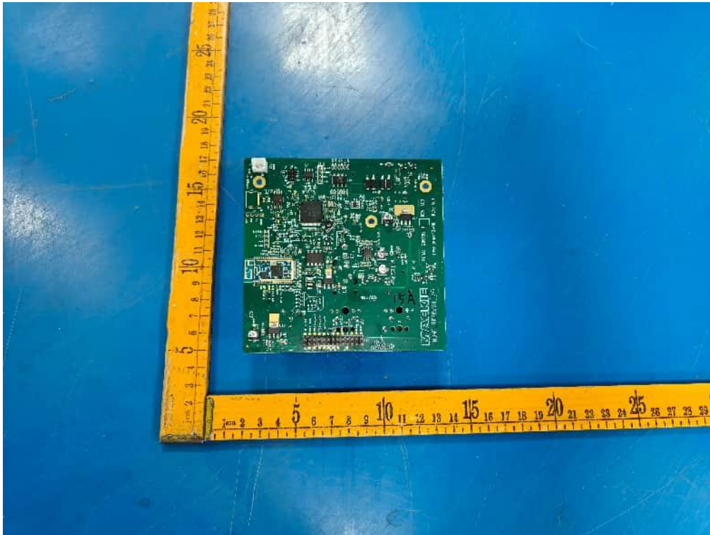
Internal view of unit (Model: THUMP15v4)
