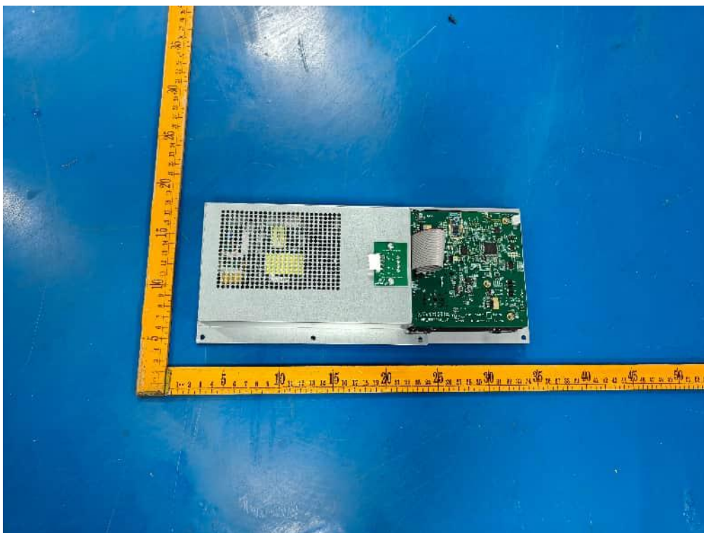
Internal view of unit (Model:THUMP12v4)
