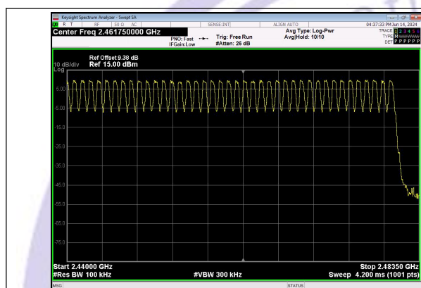
High End Spectrum Channel Hopping Plot GFSK
