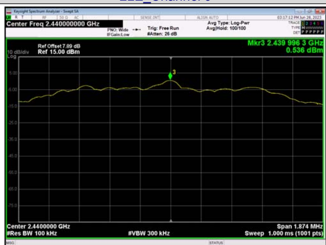
In-Band Reference Level 2LE_Channel 19
