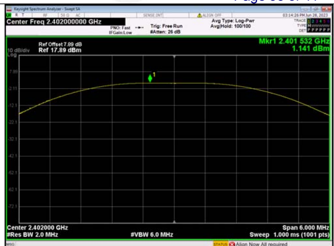
Peak Output Power 2LE_Channel 0
