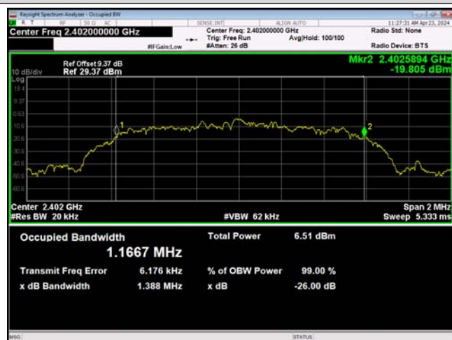
8DPSK_3-DH1_Channel 0
