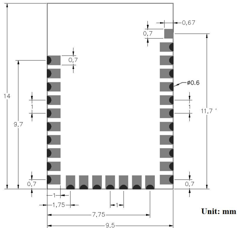
Module Dimension Diagram
