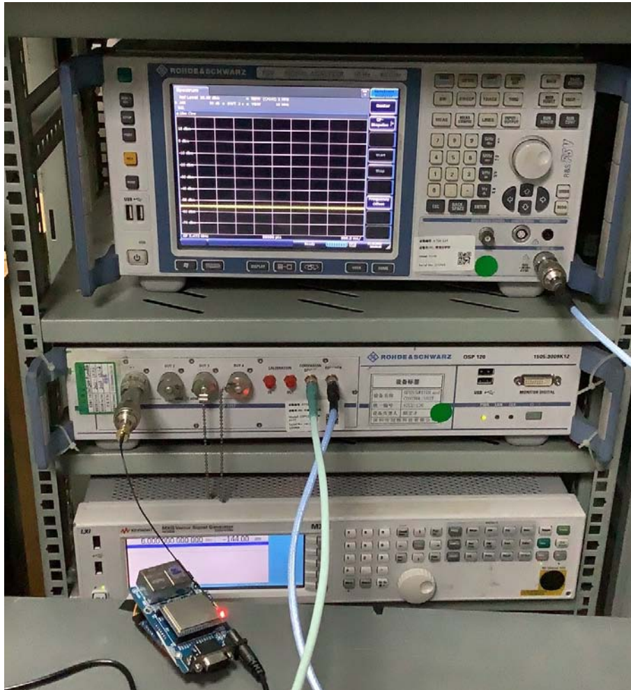
Setup photo for DFS
