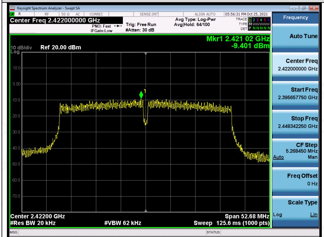
Test_Graph_802.11n40_ANT1_2422_MCS0_PSD
