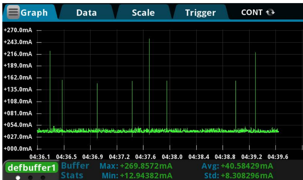
Pic 17 Bluetooth broadcast is turned on, and the module as a client keeps trying to connect to the working current of the remote server
