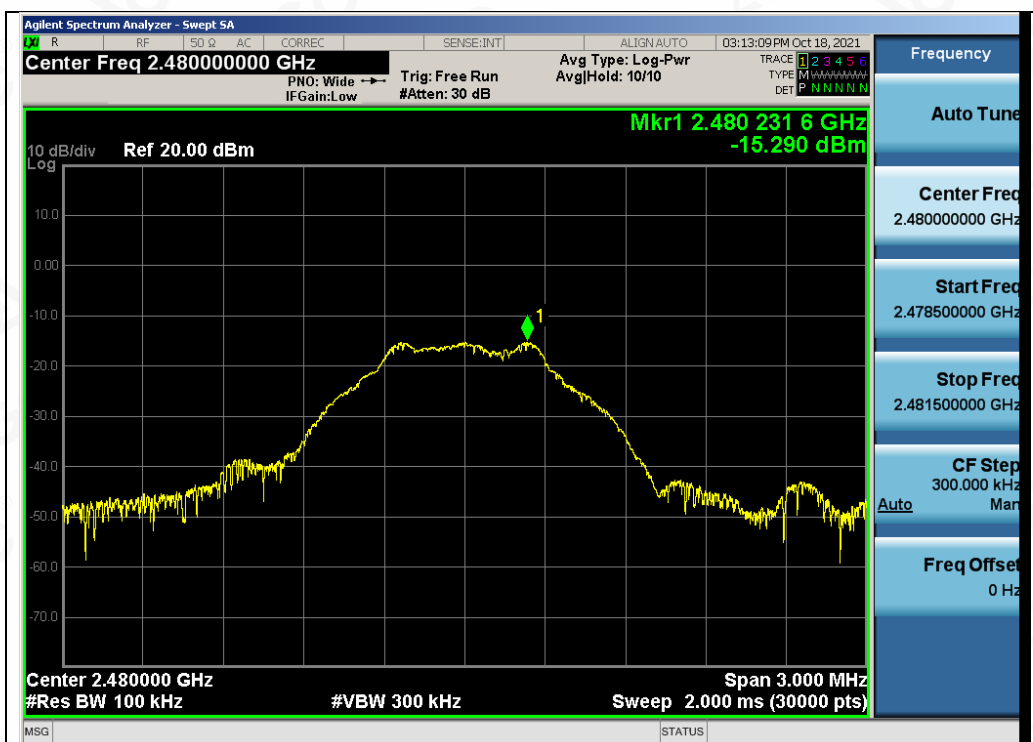
Test_Graph_LE1M_ANT1_2480_1Mbps_Reference Level
