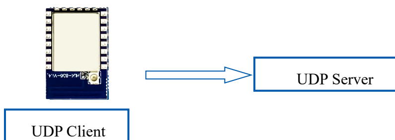
Figure 12 UDP Client
