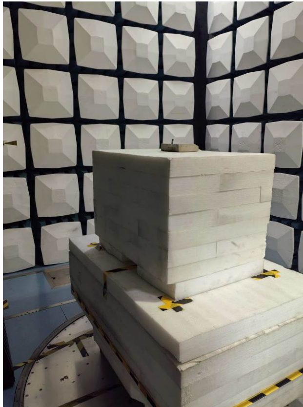
Radiated Emission 90-100GHz View
