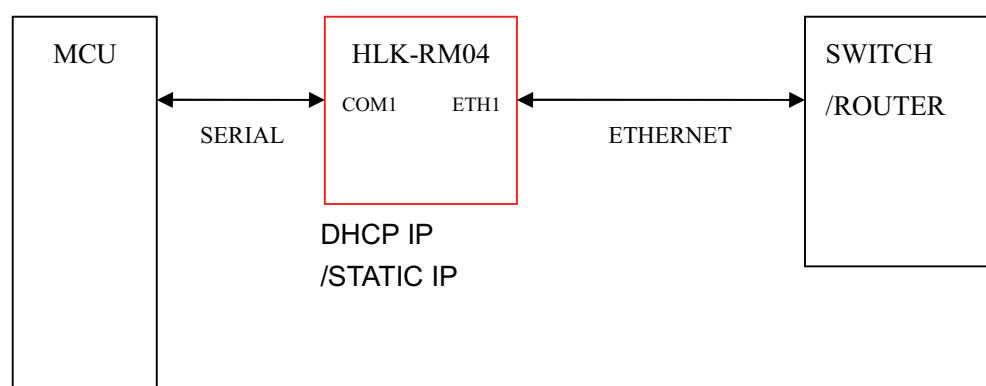
Chart3.serial to Ethernet model
