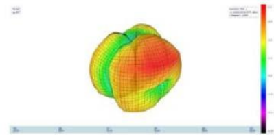
2.5Ghz 2.51dBi
