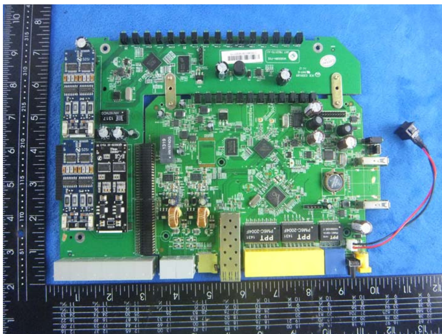
Top View of Mainboard
