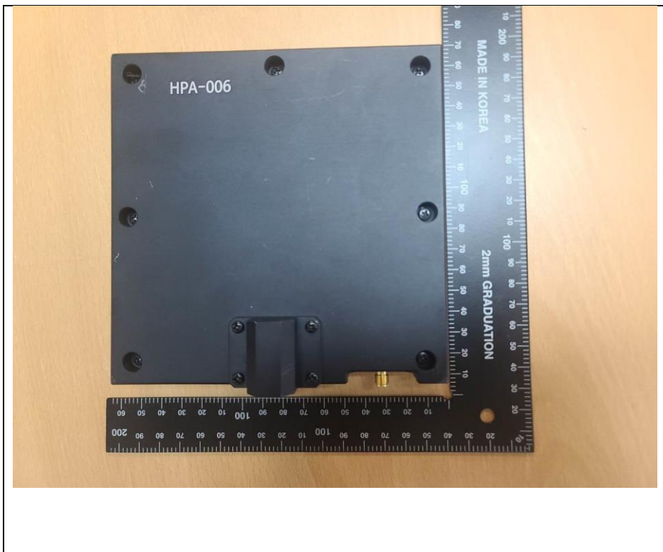
< Antenna rear View >
