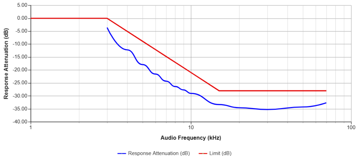
Audio Frequency Low Pass Filter Response
