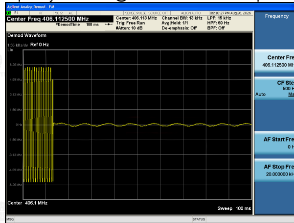
Transmitter Frequency Behavior @ 6.25 KHz Channel Separation-----On – Off
