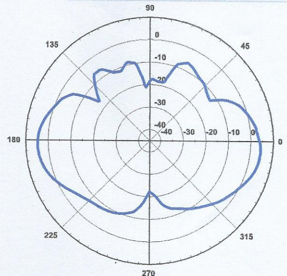
E-Plane Radiation Pattern
