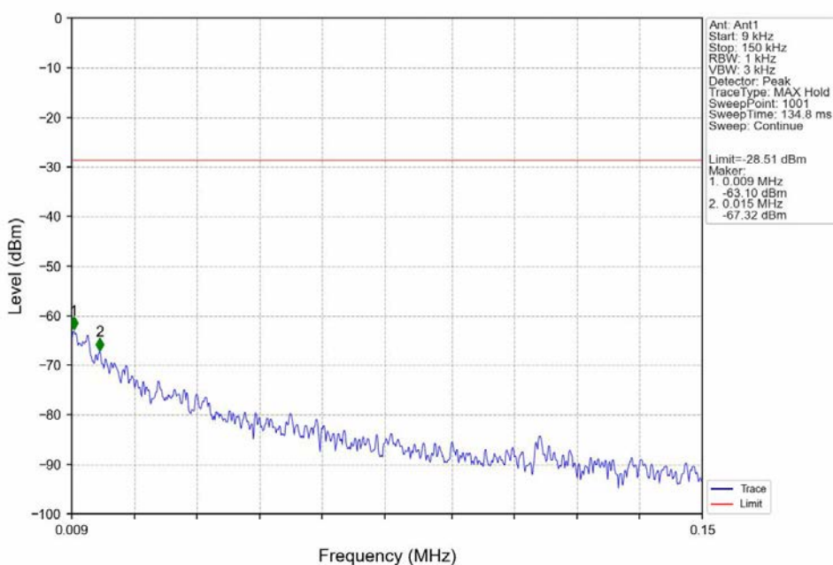
2.4G_LCH_2404.5MHz_Ant1_NTNV
