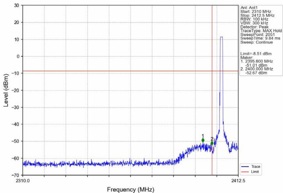
2.4G_LCH_2404.5MHz_Ant1_NTNV
