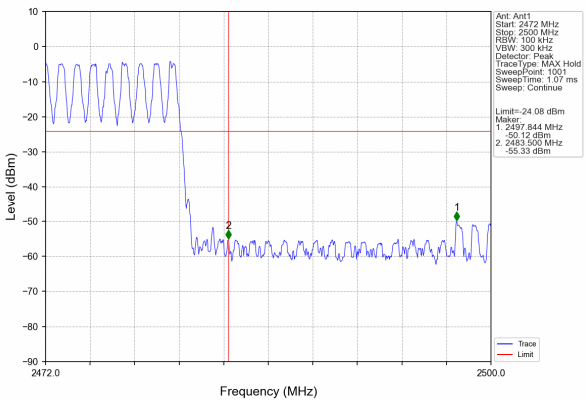
GFSK Hopping: Band edge-right side
