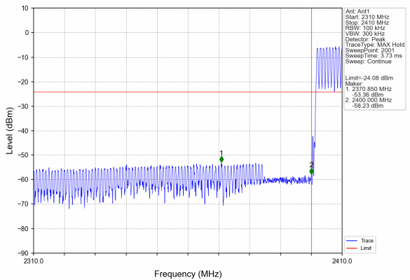
GFSK Hopping: Band edge-left side
