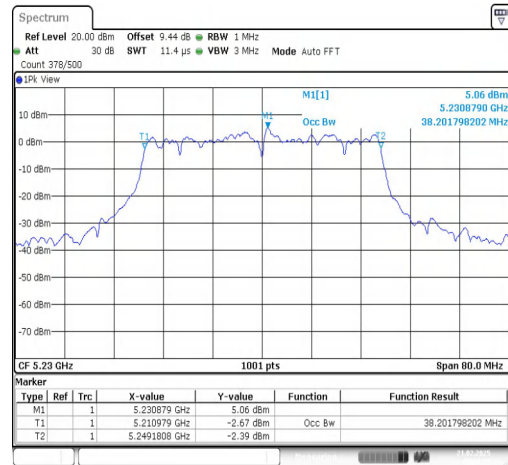
11AX40SISO-Ant1-5230
