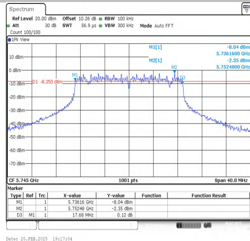
11AX20SISO-Ant1-5745-PASS
