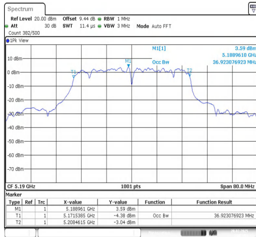
11AC40SISO-Ant1-5190
