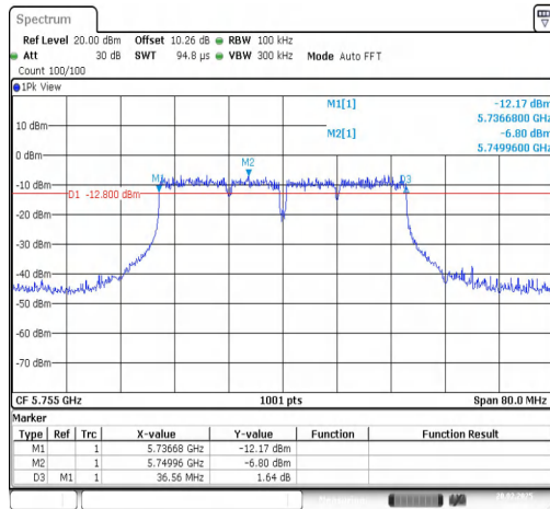
11AC40SISO-Ant1-5755-PASS
