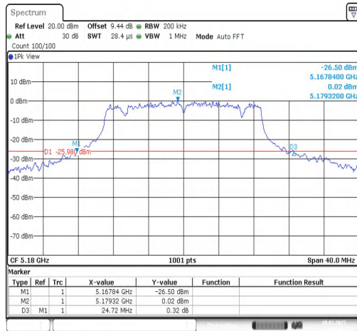
11AX20SISO-Ant1-5180
