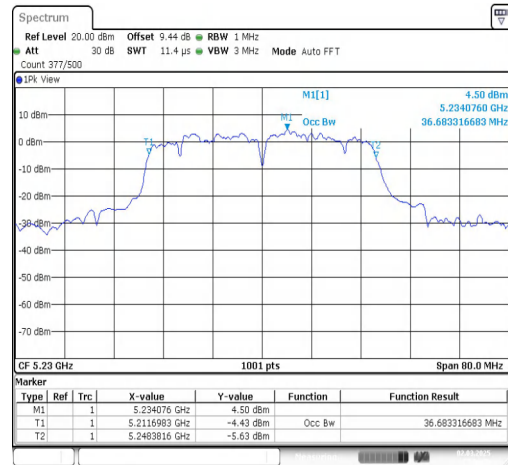
11AC40SISO-Ant1-5230
