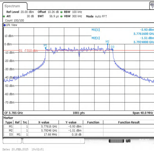
11AC20SISO-Ant1-5785-PASS
