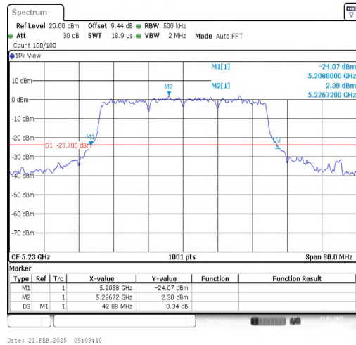
11AX40SISO-Ant1-5230
