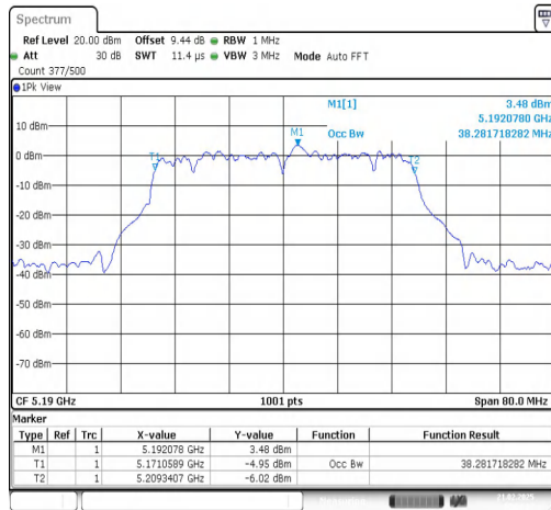
11AX40SISO-Ant1-5190
