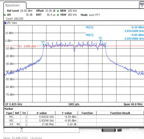
11AX20SISO-Ant1-5825-PASS
