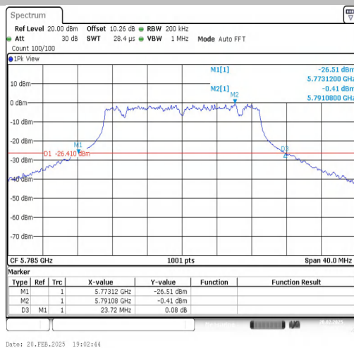
11AC20SISO-Ant1-5785
