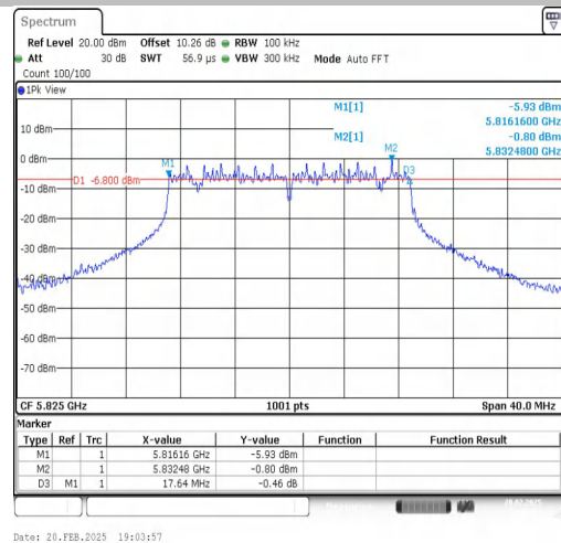
11AC20SISO-Ant1-5825-PASS
