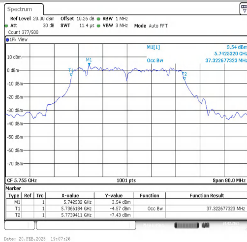
11AC40SISO-Ant1-5755
