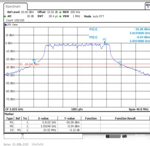
11AC20SISO-Ant1-5825
