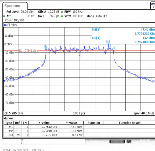
11AX20SISO-Ant1-5785-PASS
