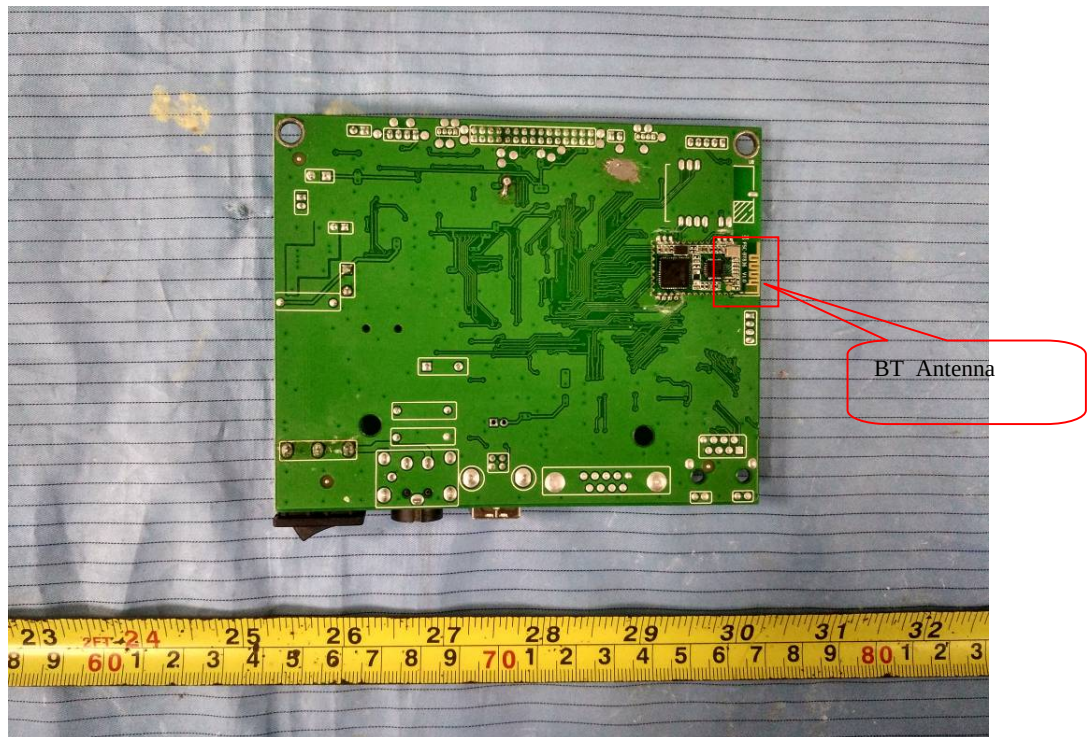
EUT – Mainboard 1 Bottom View
