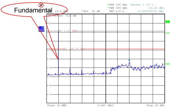
Mode: channel 39
