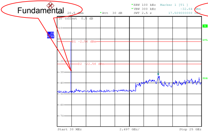
Mode: channel 0
