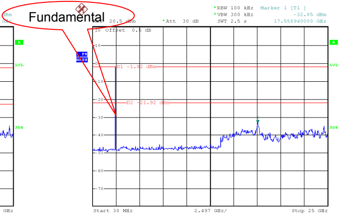
Mode: channel 19
