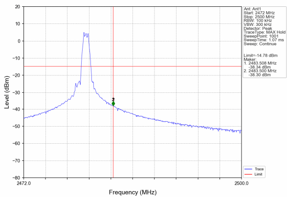
LE: Band edge-right side
