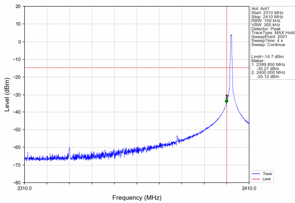
GFSK Hopping: Band edge-left side
