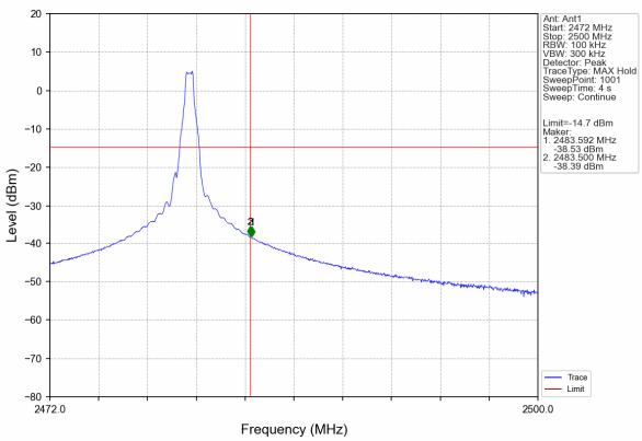
GFSK Hopping: Band edge-right side
