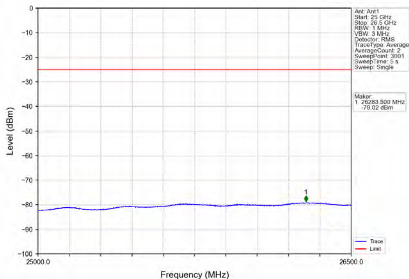
Band7 10MHz 16QAM HCH 2565MHz RB 1 0 NTNV
