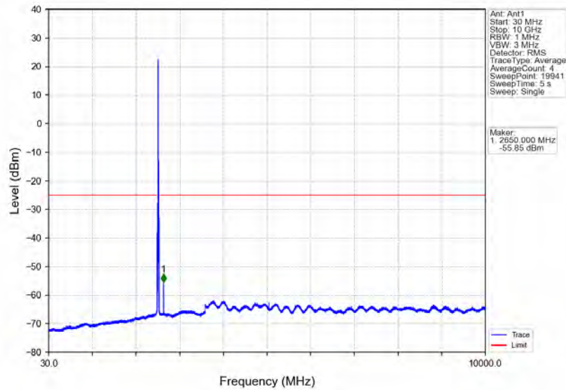
Band7_15MHz_16QAM_MCH_2535MHz_RB_1_0_NTNV
