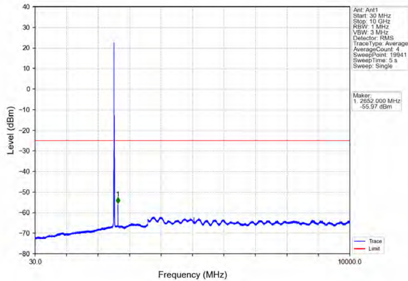
Band7_10MHz_16QAM_MCH_2535MHz_RB_1_0_NTNV
