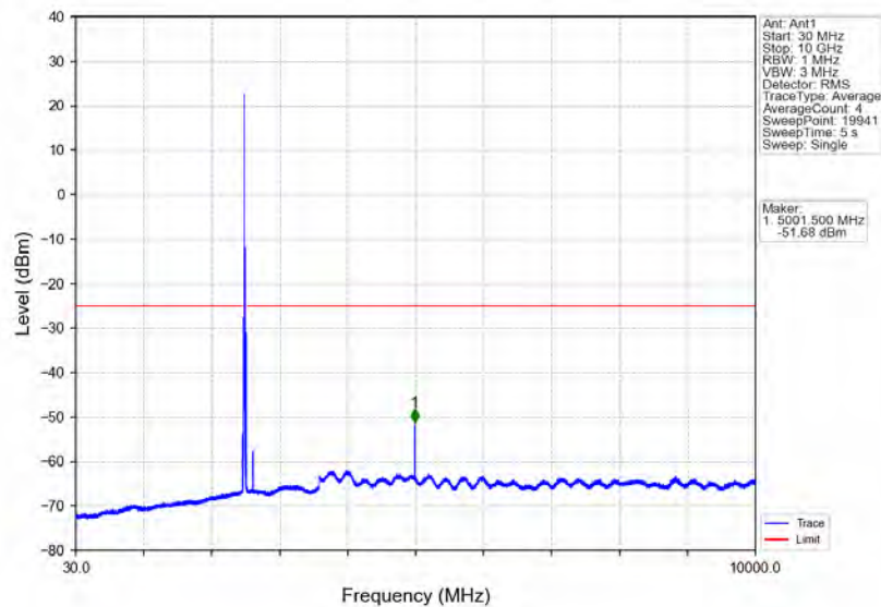
Band7_15MHz_16QAM_LCH_2507.5MHz_RB_1_0_NTNV
