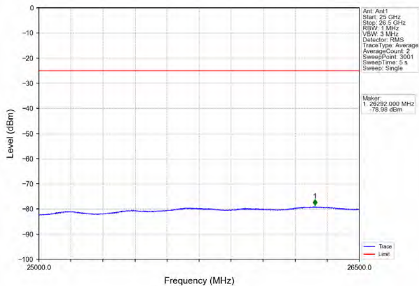
Band7 5MHz 16QAM LCH 2502.5MHz RB 25 0 NTV
