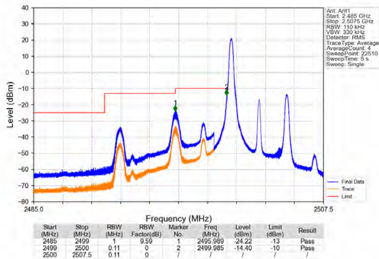
Band7_5MHz_16QAM_LCH_2502.5MHz_RB_1_0_NTNV
