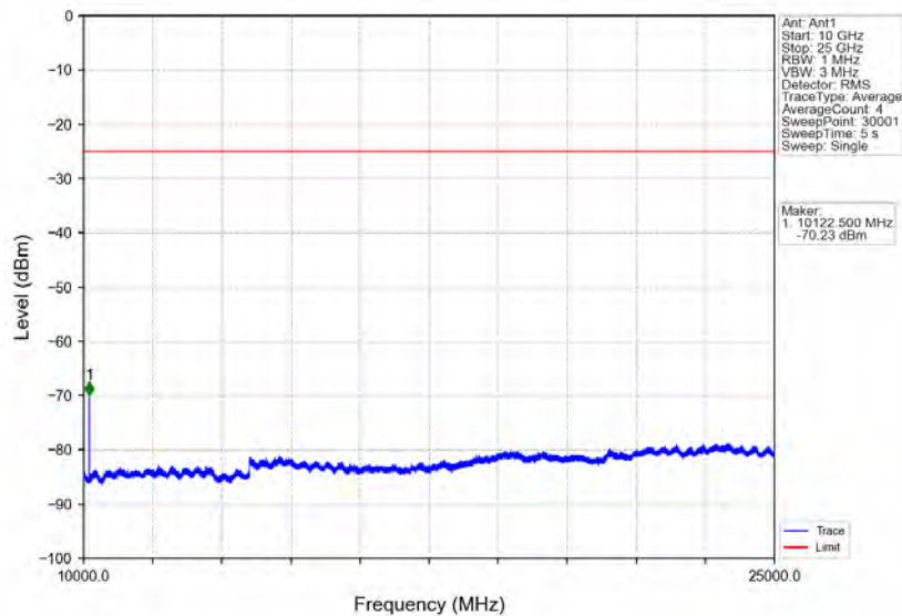
Band7_10MHz_16QAM_MCH_2535MHz_RB_1_0_NTNV
