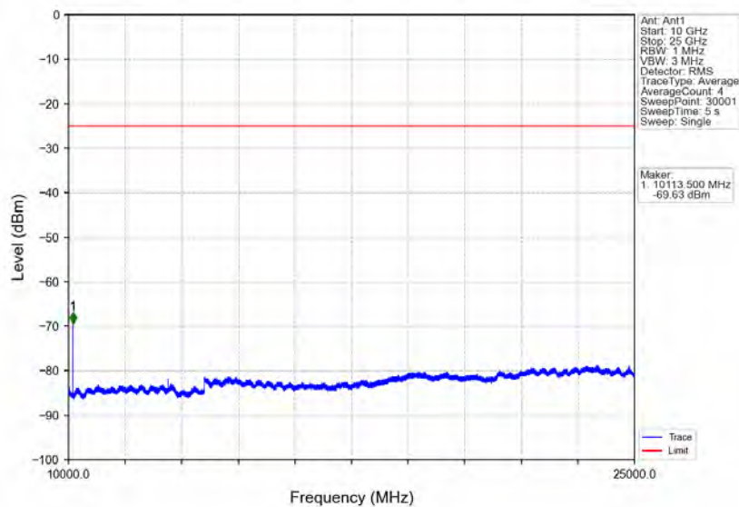
Band7_15MHz_16QAM_MCH_2535MHz_RB_1_0_NTNV
