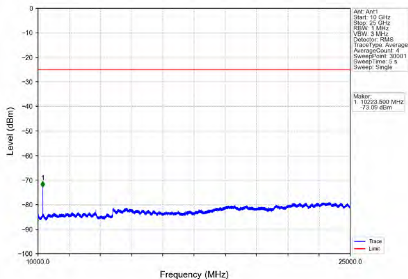
Band7_15MHz_QPSK_HCH_2562.5MHz_RB_1_0_NTV
