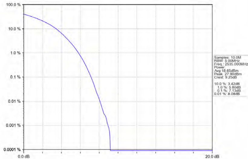
Band7_15MHz_16QAM_MCH_2535MHz_RB_75_0_NTNV
