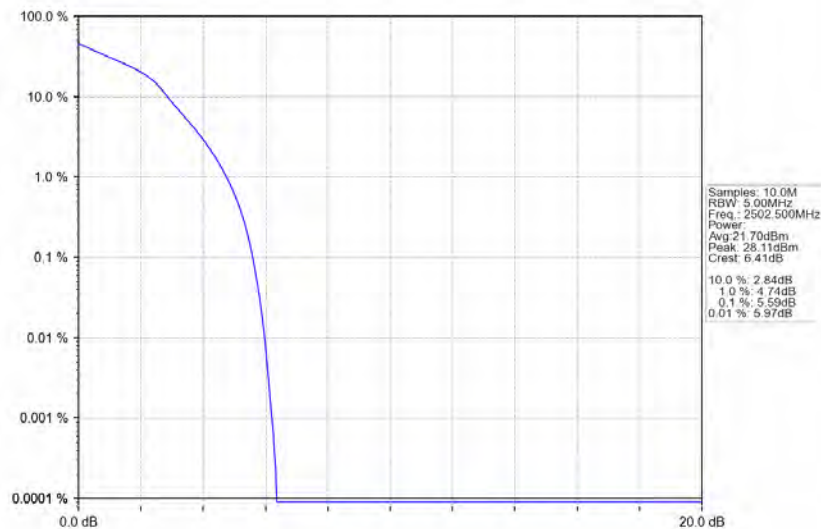
Band7_5MHz_16QAM_LCH_2502.5MHz_RB_25_0_NTNV
