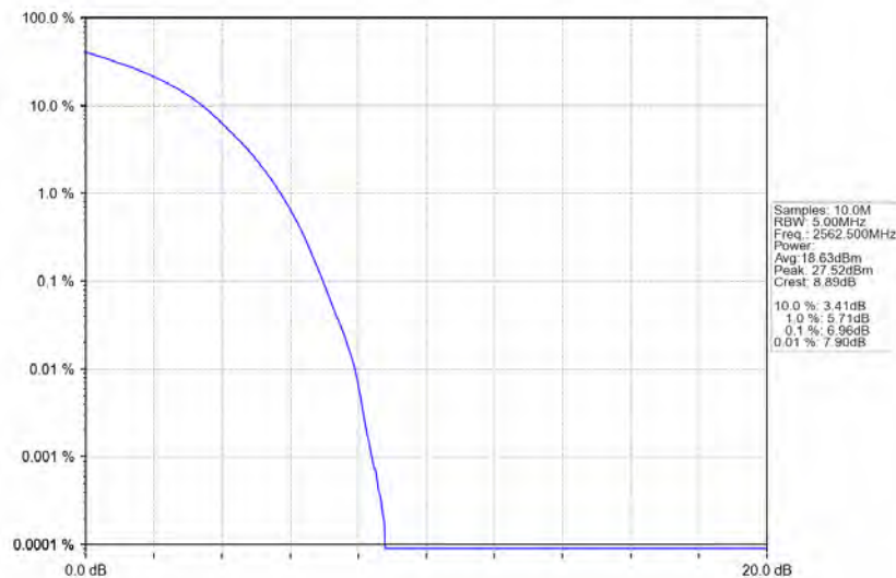
Band7_15MHz_16QAM_HCH_2562.5MHz_RB_75_0_NTNV
