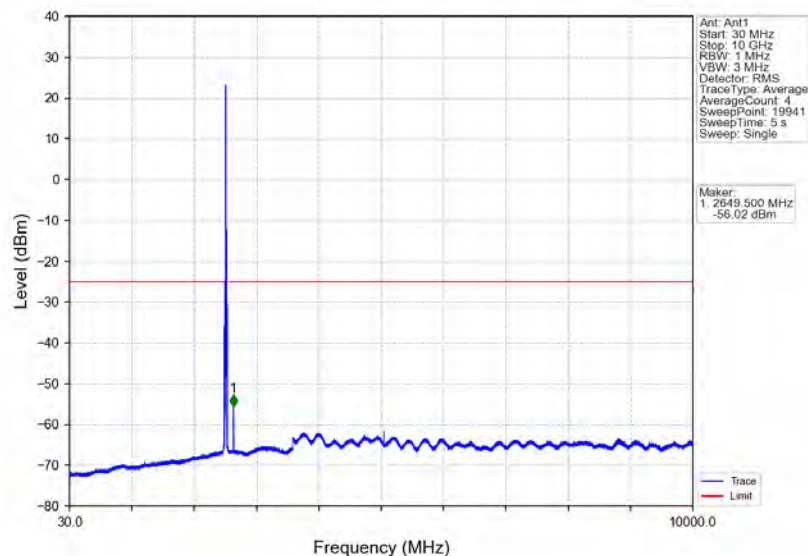
Band7_15MHz_QPSK_MCH_2535MHz_RB_1_0_NTNV
