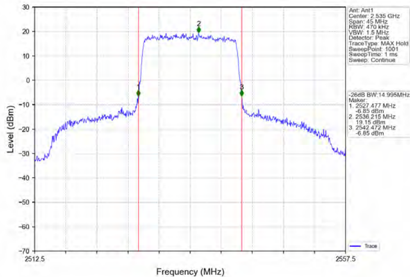
Band7_15MHz_QPSK_MCH_2535MHz_RB_75_0_NTNV
