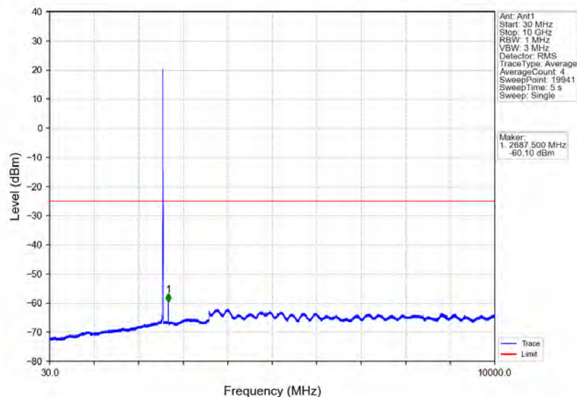
Band7_5MHz_16QAM_HCH_2567.5MHz_RB_1_0_NTNV
