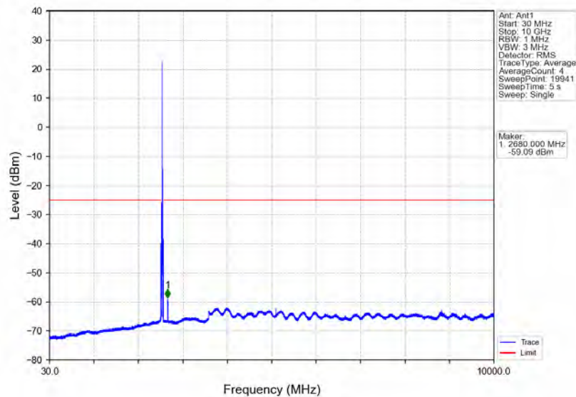
Band7_15MHz_QPSK_HCH_2562.5MHz_RB_1_0_NTV
