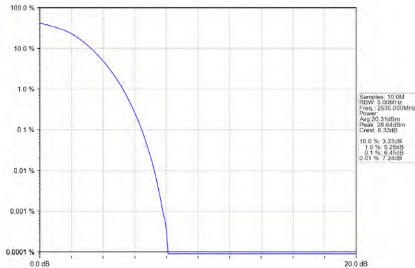
Band7_10MHz_16QAM_MCH_2535MHz_RB_50_0_NTNV
