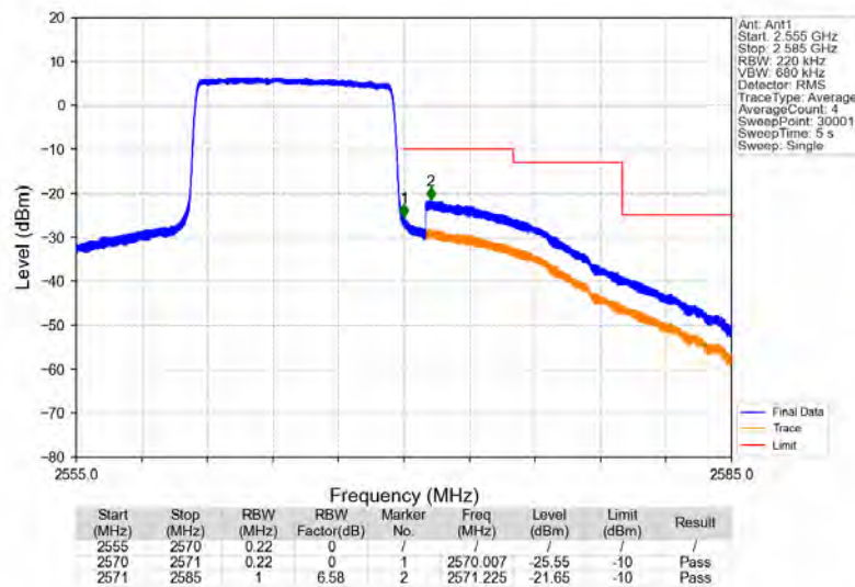
Band7 10MHz 16QAM HCH 2565MHz RB 50 0 NTNV
