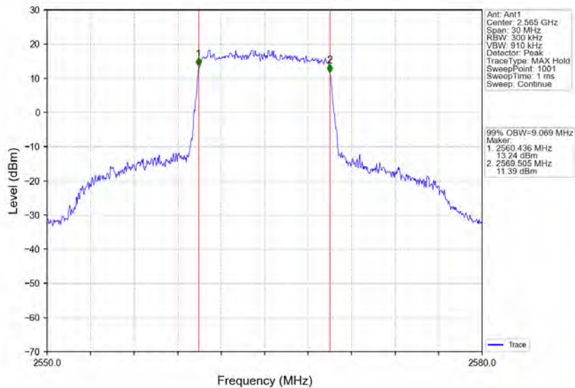
Band7_10MHz_16QAM_HCH_2565MHz_RB_50_0_NTNV
