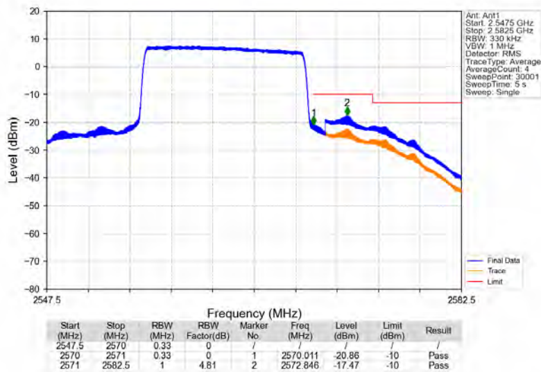
Band7_15MHz_QPSK_HCH_2562.5MHz_RB_75_0_NTNV
