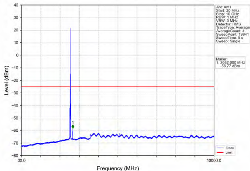
Band7_15MHz_16QAM_HCH_2562.5MHz_RB_1_0_NTNV
