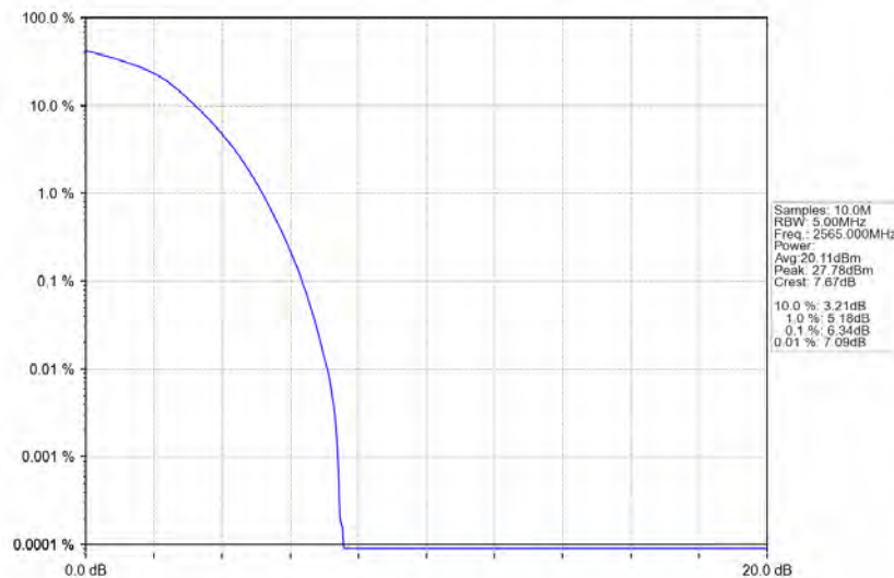
Band7_10MHz_16QAM_HCH_2565MHz_RB_50_0_NTNV
