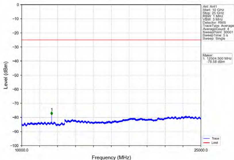
Band7_15MHz_16QAM_LCH_2507.5MHz_RB_1_0_NTNV
