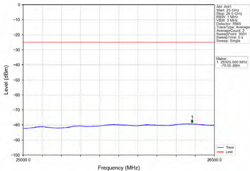
Band7_15MHz_16QAM_HCH_2562.5MHz_RB_1_0_NTNV
