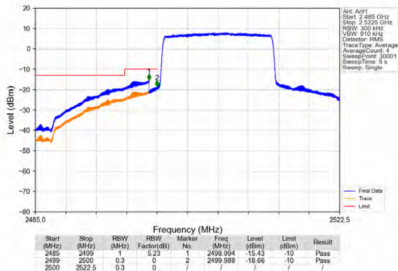
Band7_15MHz_QPSK_LCH_2507.5MHz_RB_75_0_NTNV
