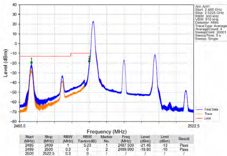
Band7_15MHz_16QAM_LCH_2507.5MHz_RB_1_0_NTNV
