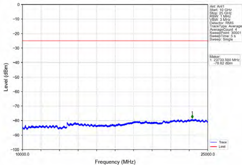
Band7_5MHz_16QAM_HCH_2567.5MHz_RB_1_0_NTNV
