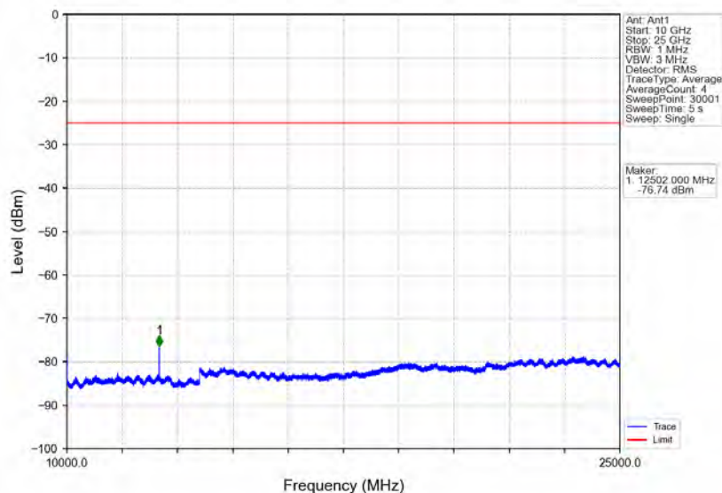
Band7 5MHz 16QAM LCH 2502.5MHz RB 1 0 NTNV
