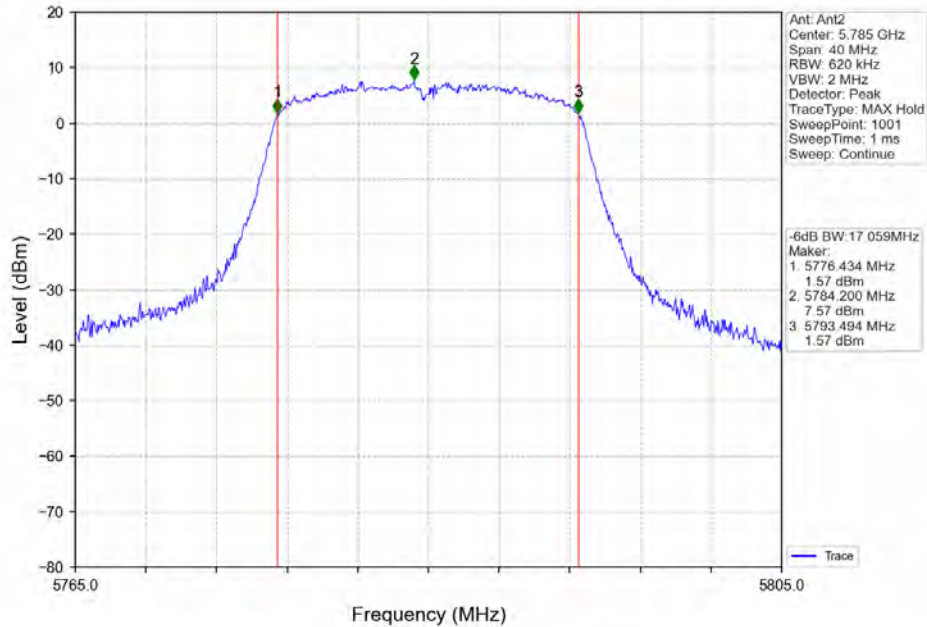
802.11ac(VHT20)_MCH_5785MHz_Ant2_NTNV
