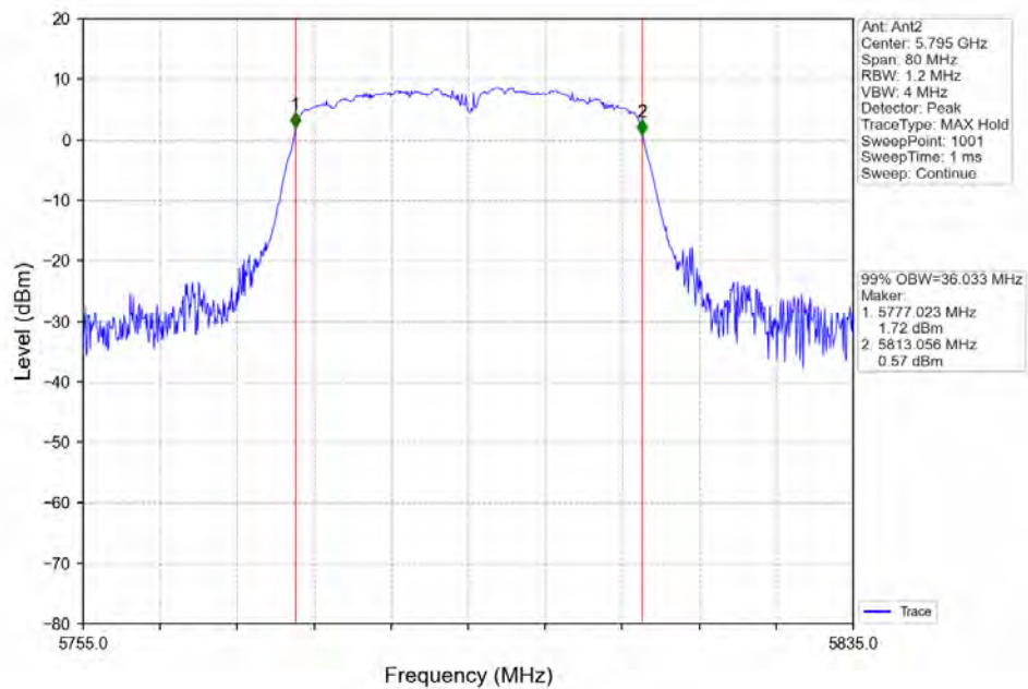
802.11ac(VHT40)_HCH_5795MHz_Ant2_NTNV
