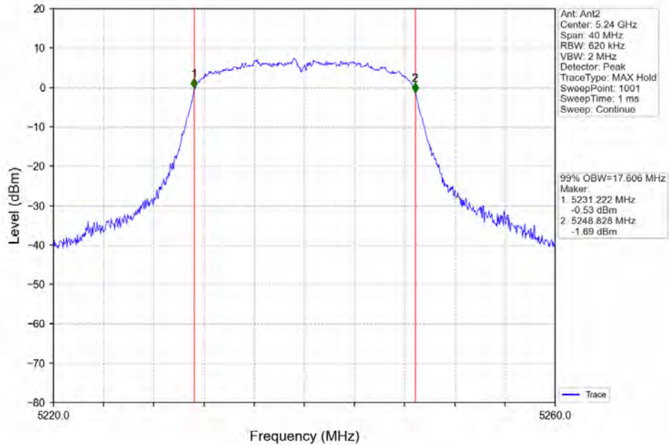
802.11ac(VHT20)_HCH_5240MHz_Ant2_NTNV
