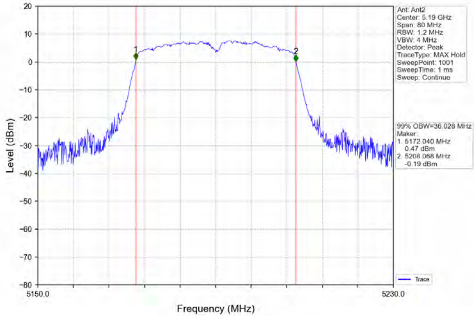
802.11ac(VHT40)_LCH_5190MHz_Ant2_NTNV
