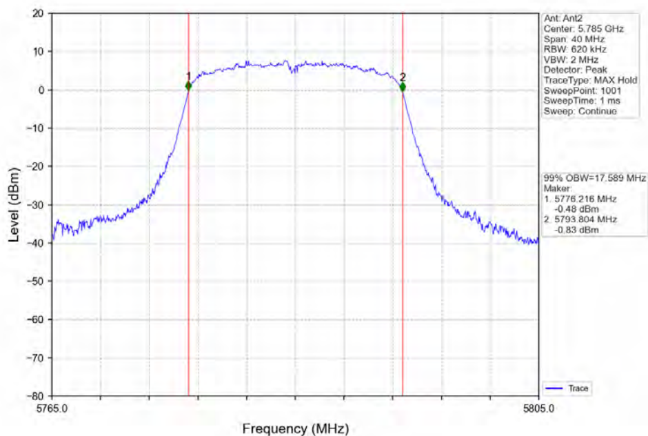
802.11ac(VHT20)_MCH_5785MHz_Ant2_NTNV
