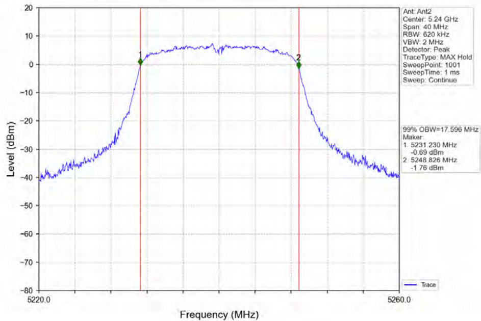
802.11n(HT20)_HCH_5240MHz_Ant2_NTNV
