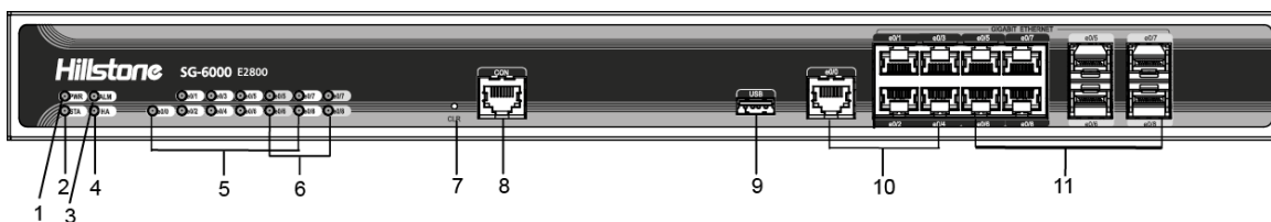
Figure 1-8: Front Panel of SG-6000-E2800 and SG-6000-E2300
