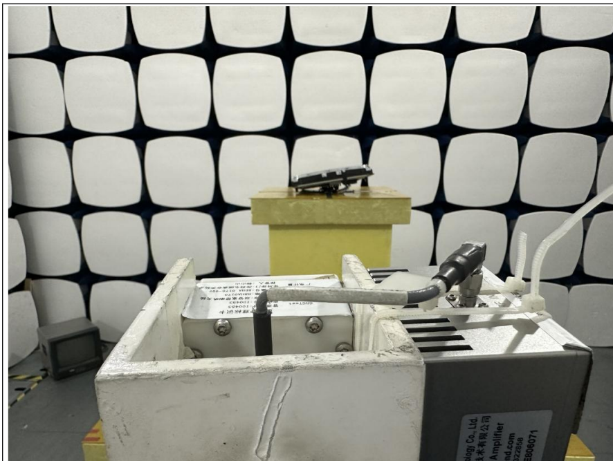
18GHz-26.5GHz (BT&BLE)
