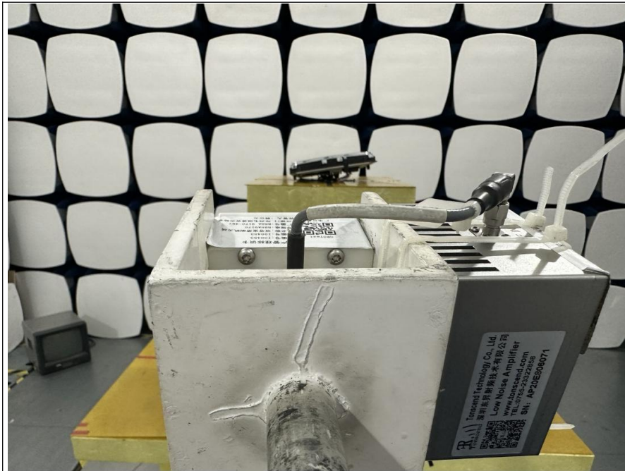
18GHz-40GHz (WiFi)
