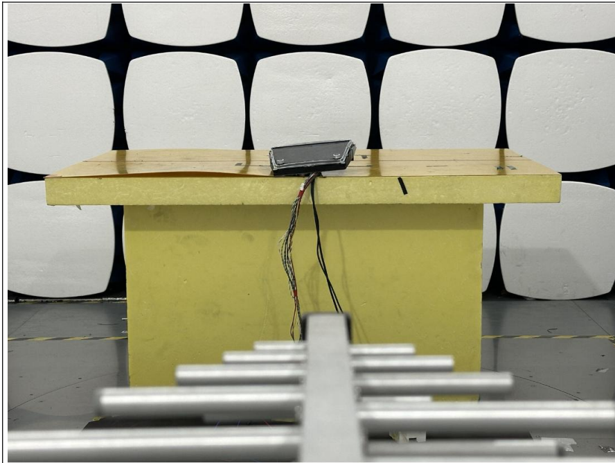
30MHz-1GHz (WiFi)
