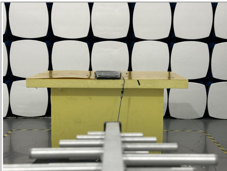
30MHz-1GHz(BT&BLE)
