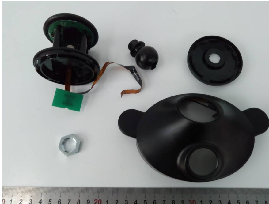
EUT –Upper Part 2 View
