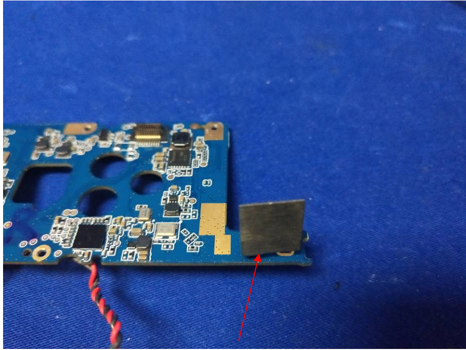
Wireless antenna
