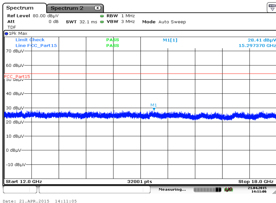
Plot 7: 12 GHz to 18 GHz, mid channel, vertical & horizontal polarization – valid for all channels
