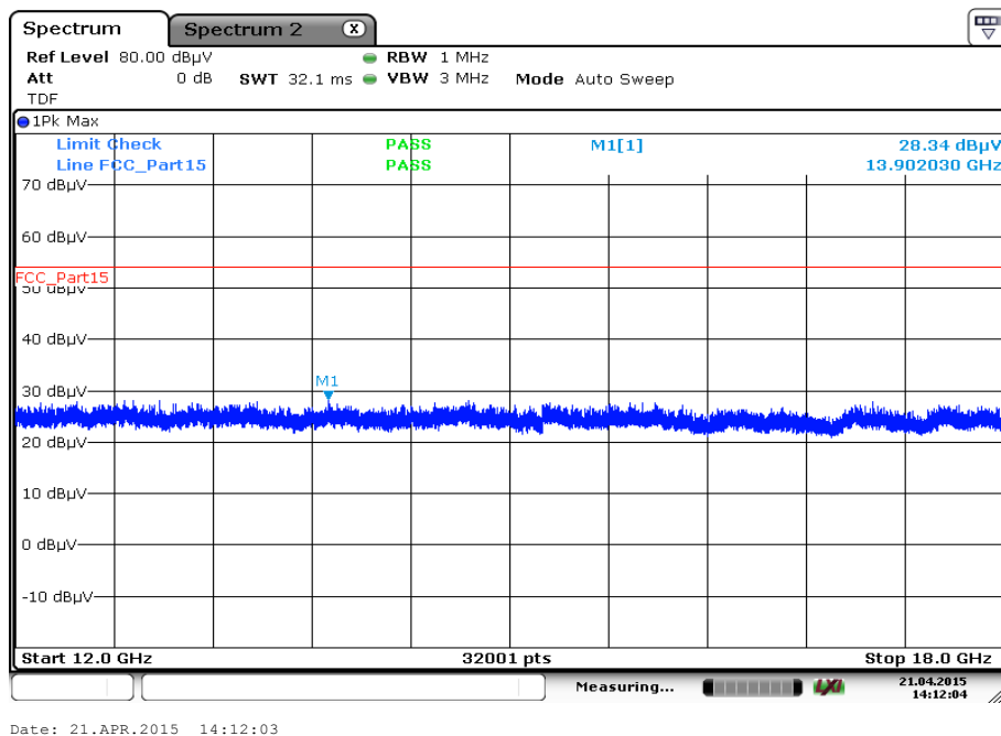
Plot 11: 12 GHz to 18 GHz, highest channel, vertical & horizontal polarization – valid for all channels
