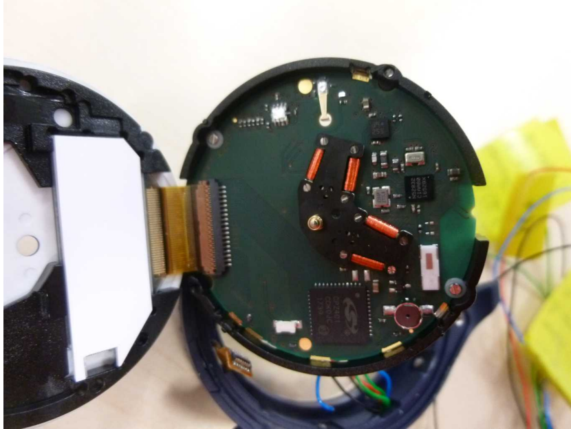
Photo 3: PCB front side view with antenna
