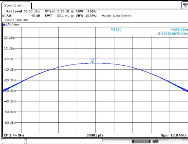
Channel 19 (2440MHz)
