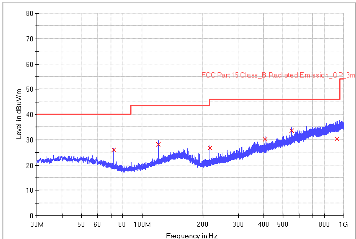
RE_VULB9168_pre_Cont_30-1000
