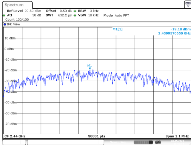
Channel 19 (2440MHz)
