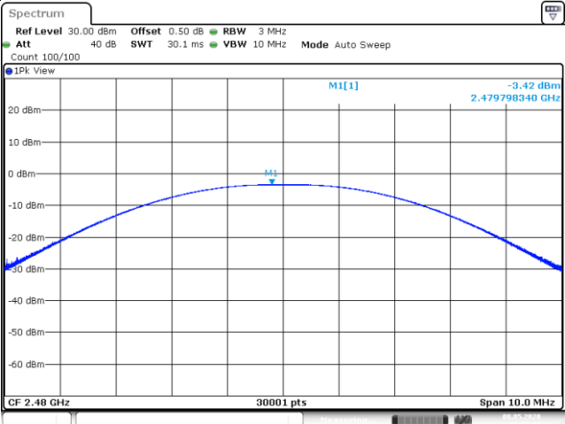
Channel 39 (2480MHz)
