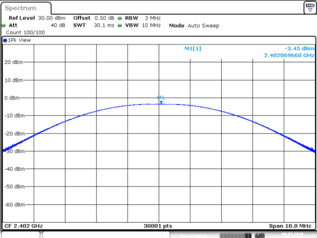
Channel 0 (2402MHz)
