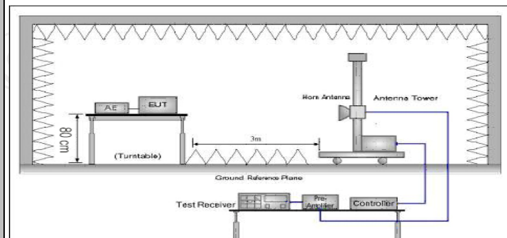
Above 1GHz
