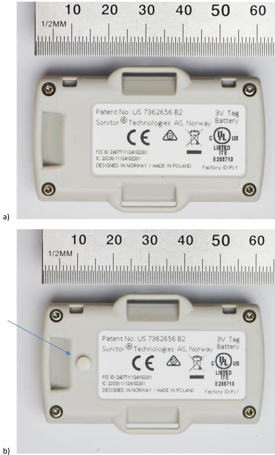
Figure 2: a) Photo of back side of Tag-M500/Tag-M501 and b) photo of back side of Tag-M503. A tamper pin is seen for the latter, as indicated with an arrow.
