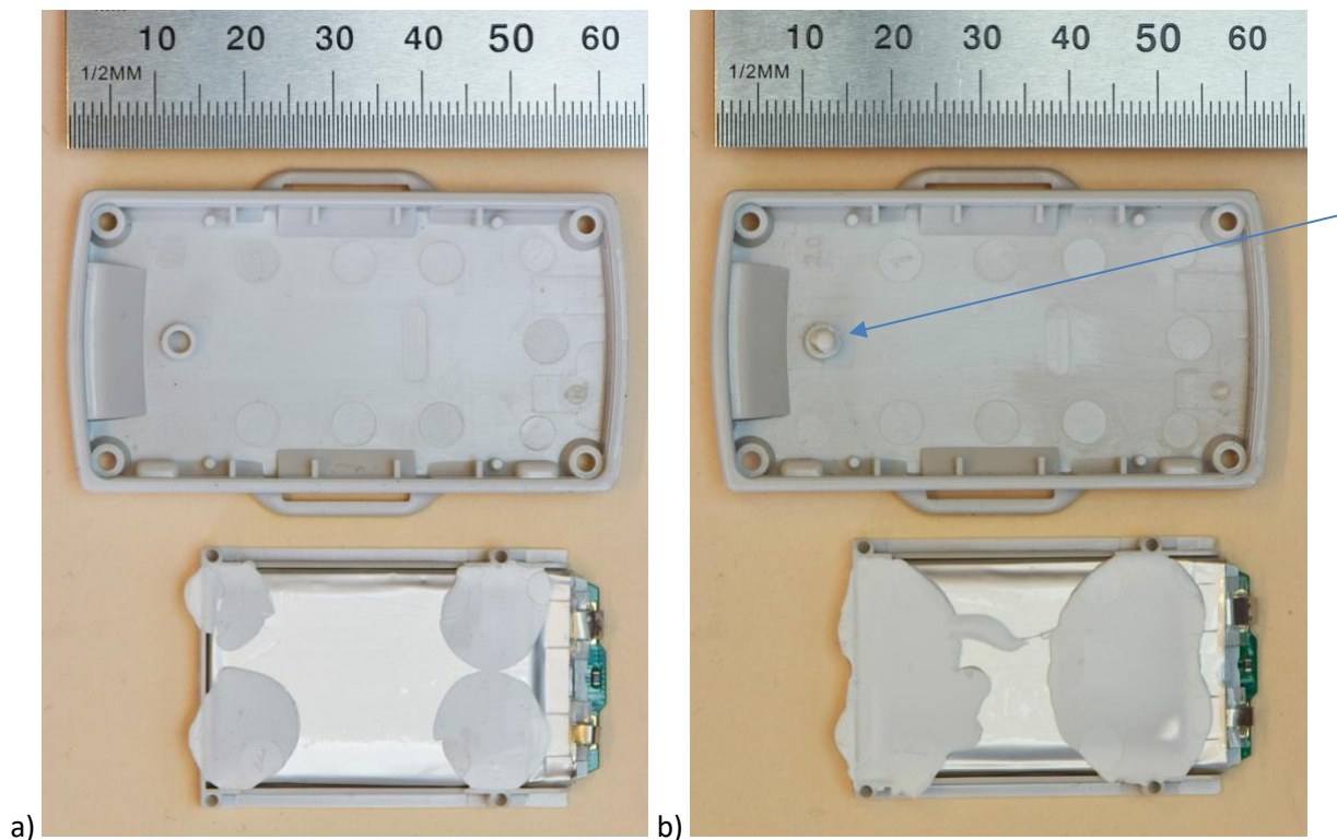
Figure 1: a) Photo of base of Tag-M500/Tag-M501 and b) of Tag-M503. In both photos, the sub-assembly containing a thin-film battery has been torn from the housing and flipped to show how it is attached to the housing using an adhesive. A tamper pin (arrow) is seen for Tag-M503.
