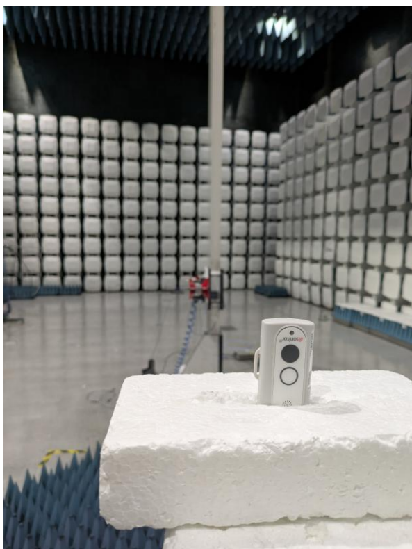
Radiated 1000-18000 MHz spurious emissions - from device
