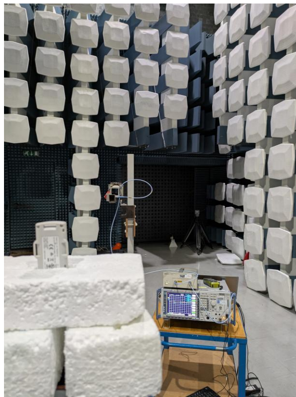
Radiated 18000-26000 MHz – from device. Spectrum analyser with preamp on table. Horn antenna on vertical stand at 1 meter distance.
