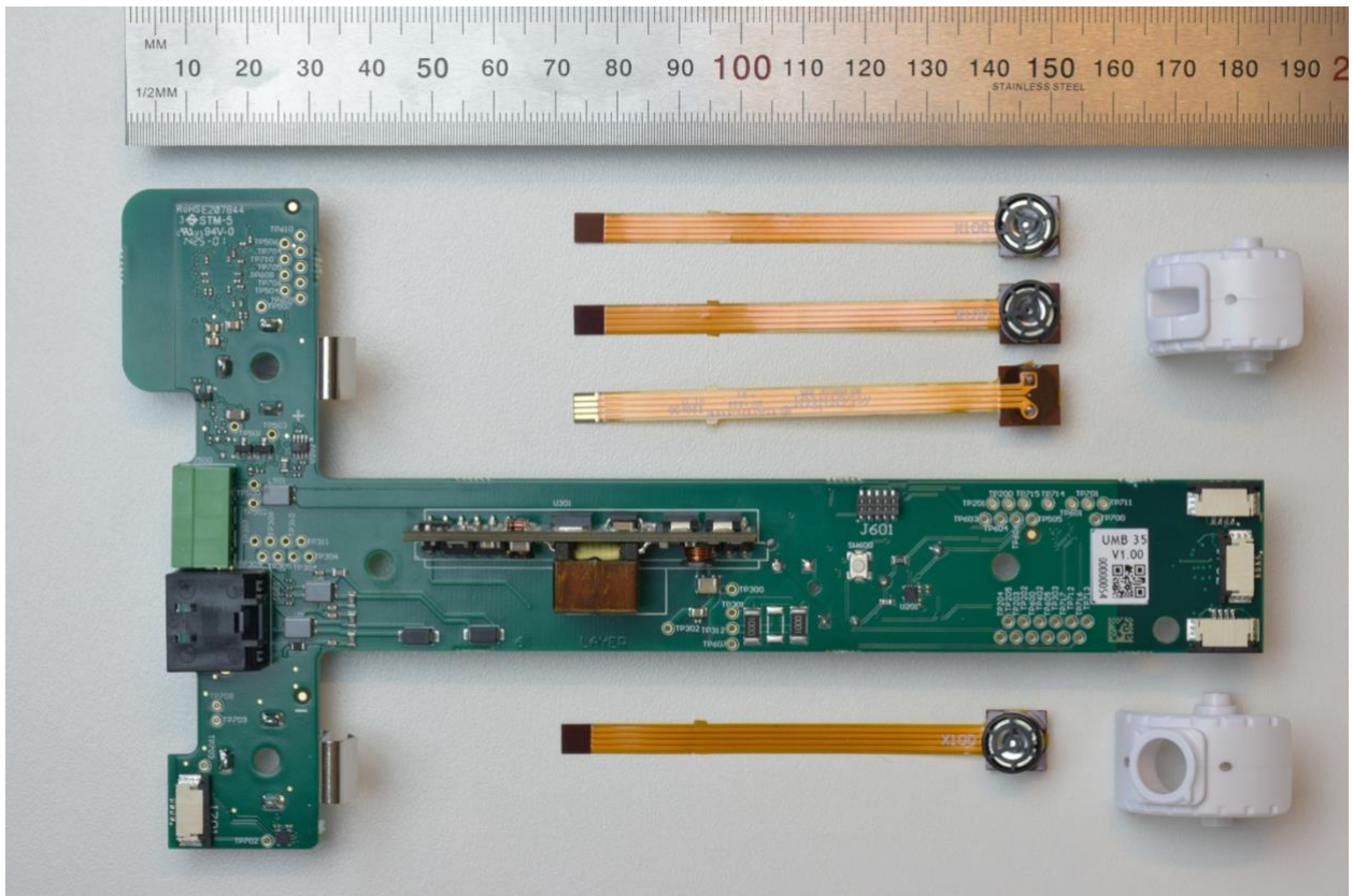
Figure 1: Photo of the PBA of INF-C39X, front. All the four ultrasound transducer subassemblies seen beside the PBA (one flipped) get mounted to the board for all models. A turret like the one seen to the upper right is mounted to each transducer for INF-C398 and INF-C399 whereas a turret like the one seen to the lower right is mounted to each transducer for INF-C396.
