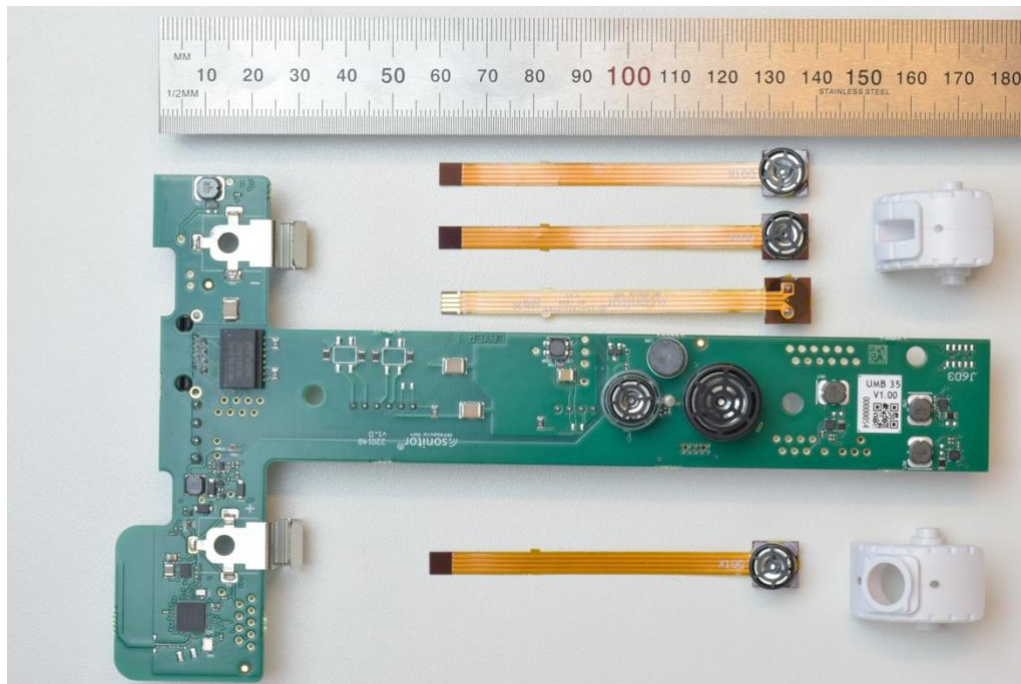
Figure 2: Photo of the PBA of INF-C39X, back.
