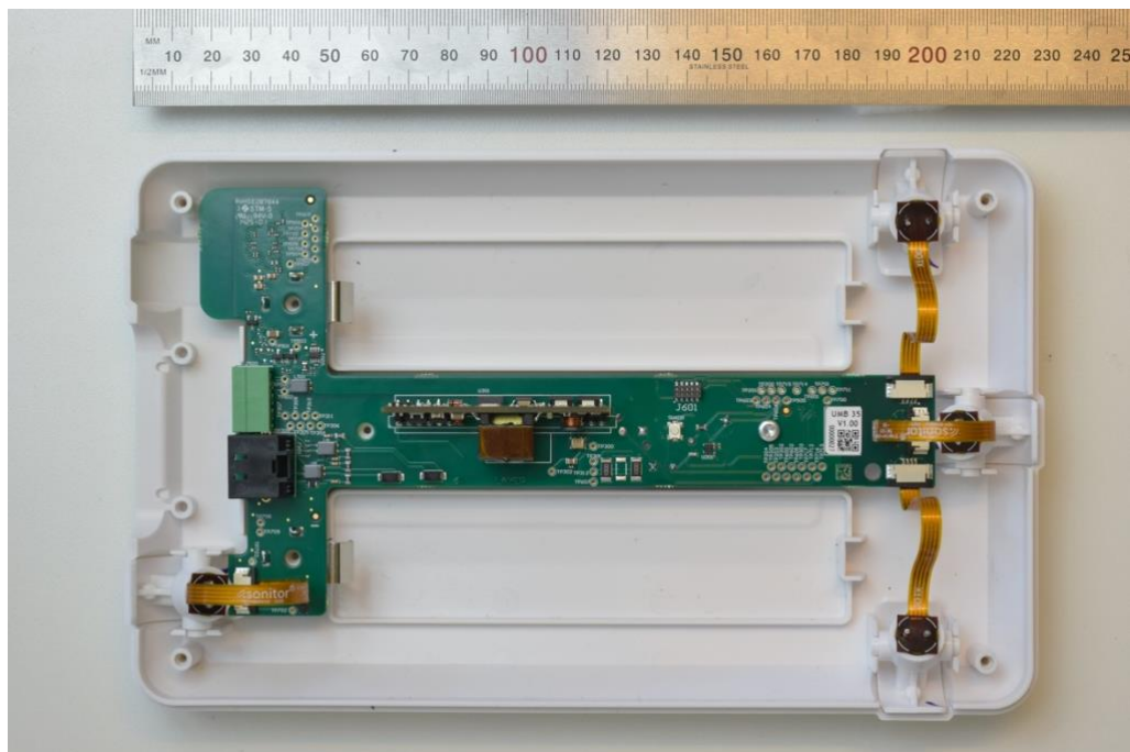
Figure 3: Photo of the PBA of INF-C39X, with ultrasound transducers mounted, mounted inside the housing.
