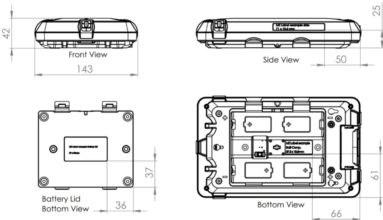
Figure 1: Illustration of label placements (all dimensions in mm). Since the Battery Lid (lower left illustration) is possible to remove, the critical safety information is replicated on a smaller label inside the housing compartment (lower right illustration).
