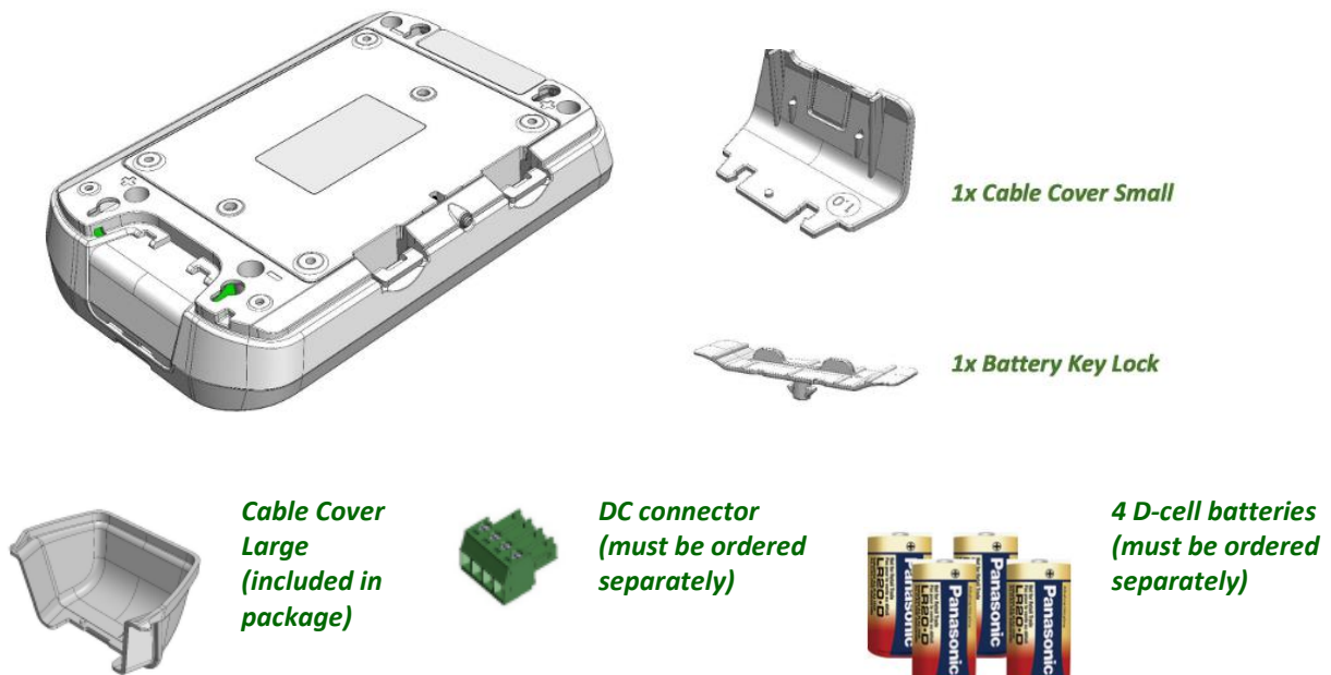
Figure 2: Parts for models INF-C39X where some parts, as indicated, are either included in the package or must be ordered separately. The Cable Cover Small and the Battery Key Lock are parts that are pre-mounted in the factory.
