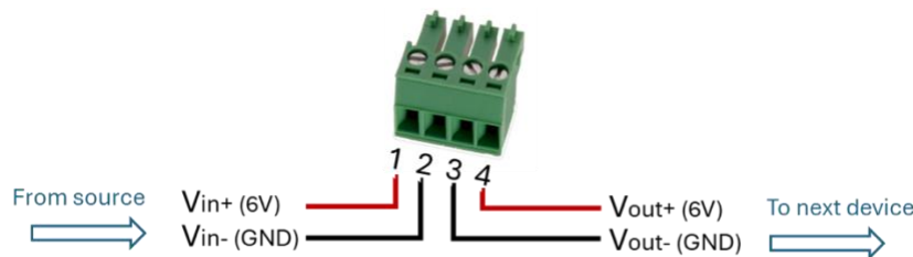
Figure 3: Overview of terminals for DC power supply.
