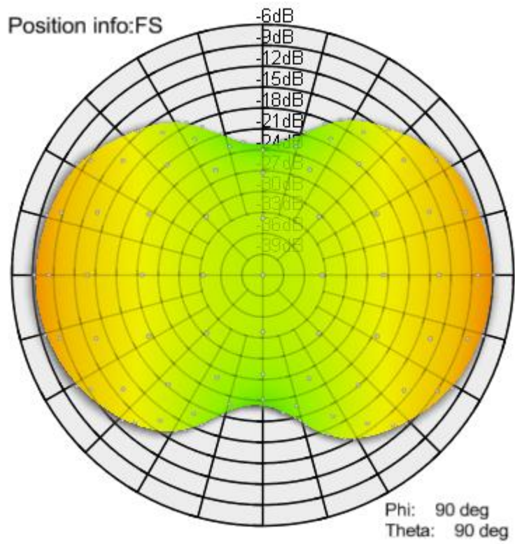
Figure 6 Antenna pattern BLE channel 38 [dBm]
