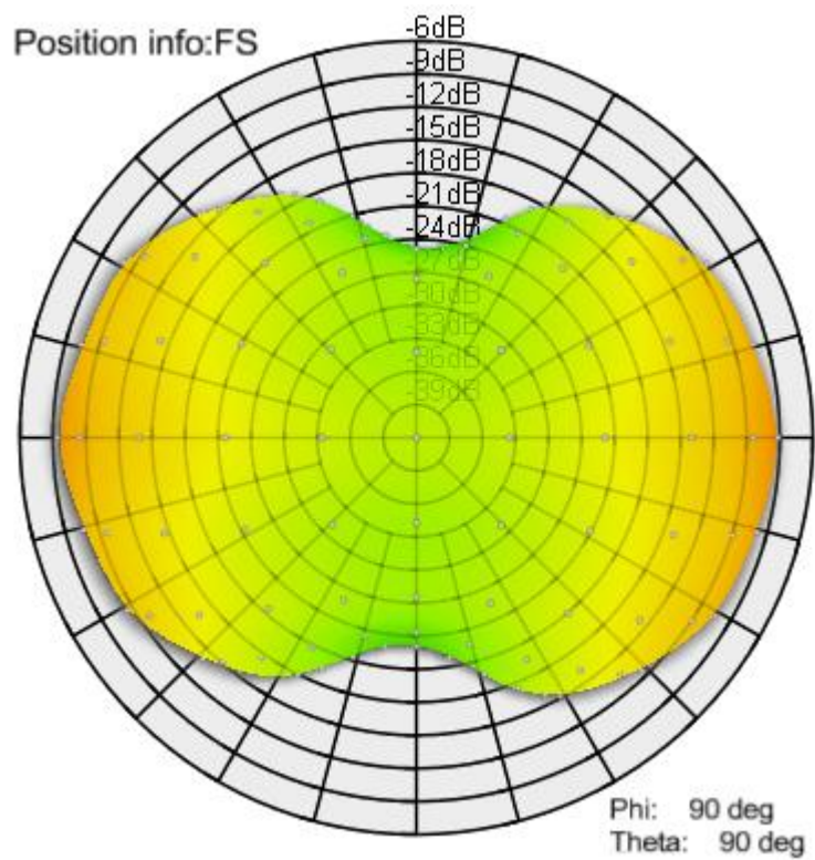
Figure 5 Antenna pattern BLE channel 37 [dBm]
