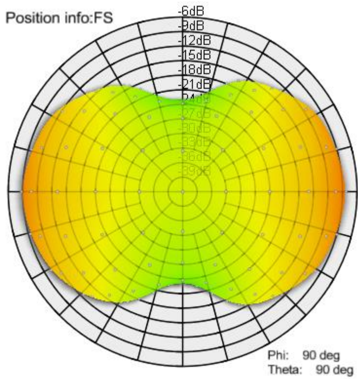
Figure 7 Antenna pattern BLE channel 39 [dBm]
