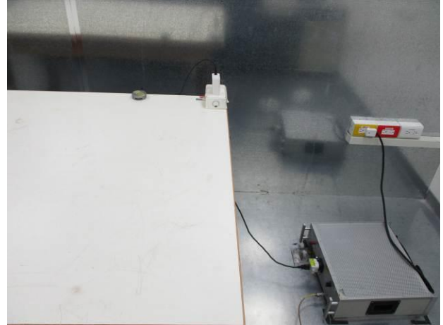
FCC_15_247_BLE_Conduction_Setup
