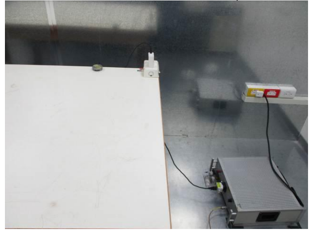
FCC_15_209_WPT_Conduction_Setup
