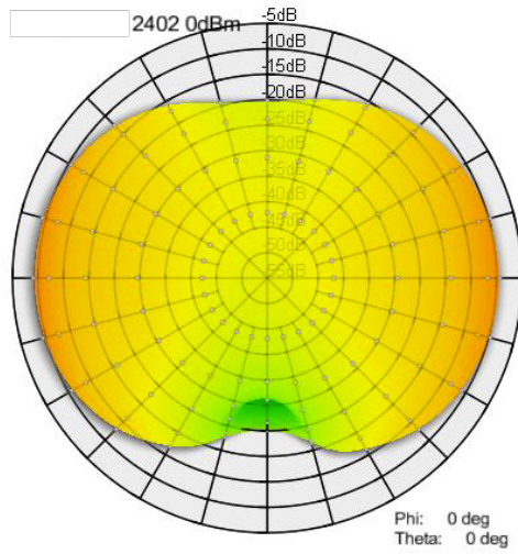
Figure 1 Antenna pattern BLE channel 37 [dBm]
