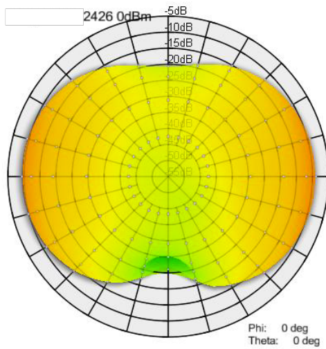
Figure 2 Antenna pattern BLE channel 38 [dBm]
