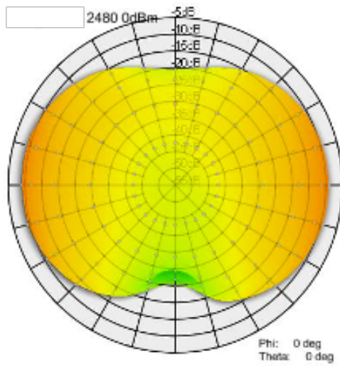
Figure 3 Antenna pattern BLE channel 39 [dBm]
